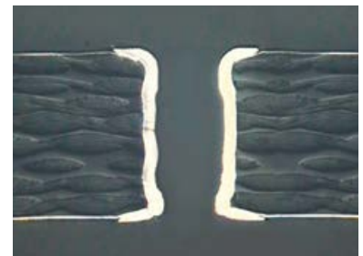
Through-hole plating with LPKF ProConduct
